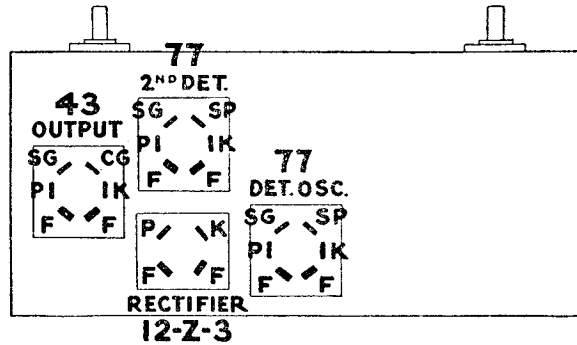
Fig. 1—Tube Sockets, Under Side of Chassis
